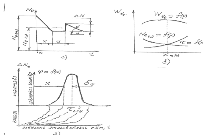
Figure 1. Variation of engine power a) productivity b) maintenance period during vehicle service as a function of maintenance period. c) Scheme for determining preventive maintenance time of vehicle
