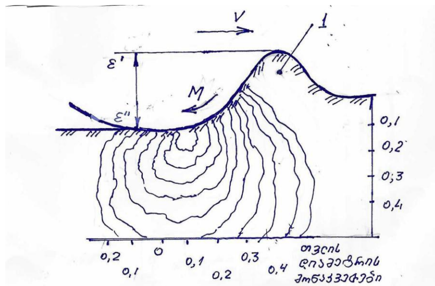
Fig. 2. Soil stress diagram under the wheel
