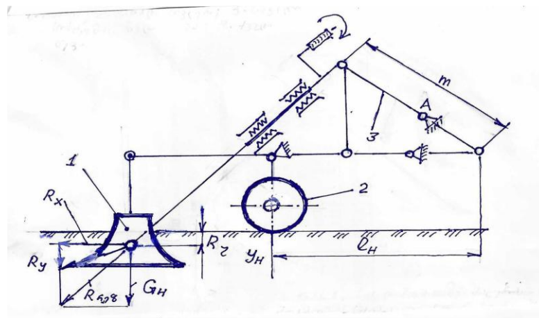
Fig.1. Forces acting on the suspension mechanism in the longitudinal plane .
