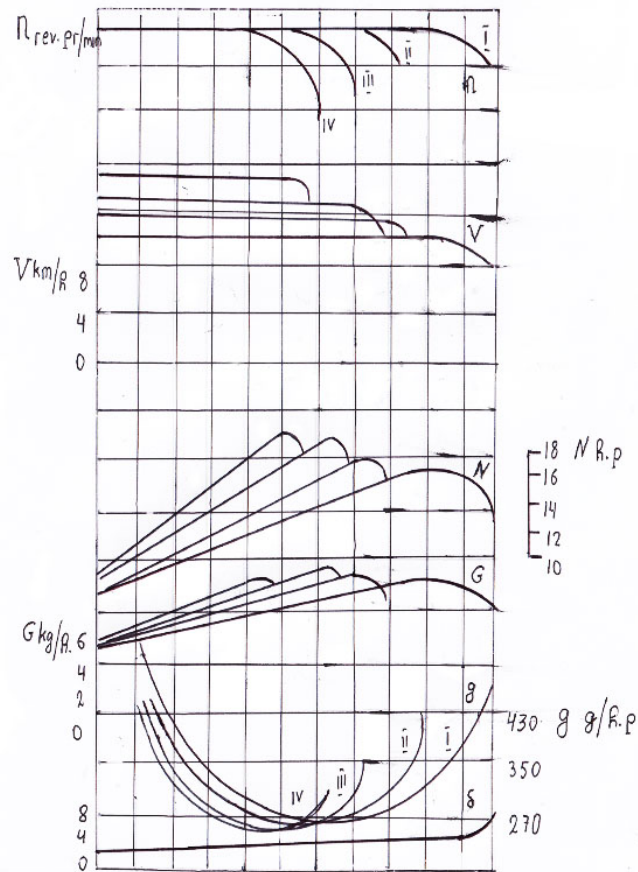
Fig. 2. Tractor traction characteristic
